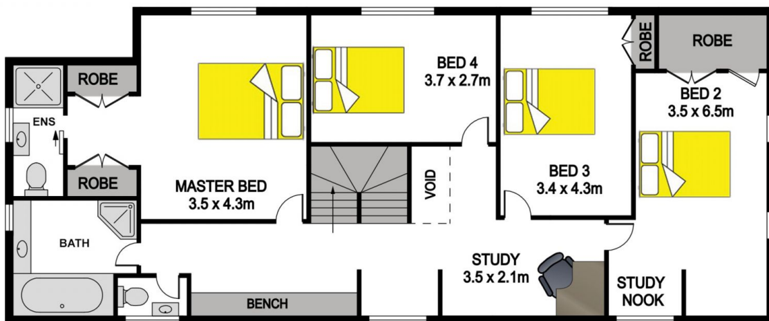
UPPER FLOOR
